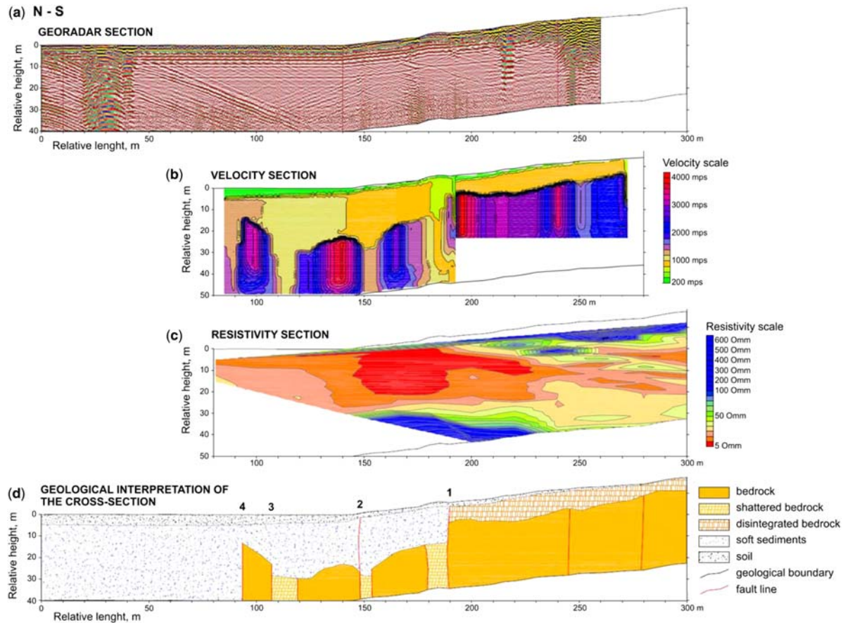
Fig. 7. Results of the geophysical profiling across the Euphrates fault zone in the southern bank of the Euphrates River, 3 km south of the town of Ar Raqqa: (a), Georadar section; (b), section of velocities of the refraction waves (the correlation refraction method); (c) geoelectric resistance section (the dipole axial sounding); and (d) geological interpretation. The visible vertical offset of the Tortonian surface is c. 15 m on the fault strand 1. The offset on strand 2 is smaller. Strand 2 ruptures the terrace I gravel and is reflected by small gentle scarp in the land surface. Strands 3 and 4 border narrow horst which is not reflected in the land surface. The total offset of the surface of the Tortonian on all strands of the Euphrates fault zone is not less than c. 25 m.
