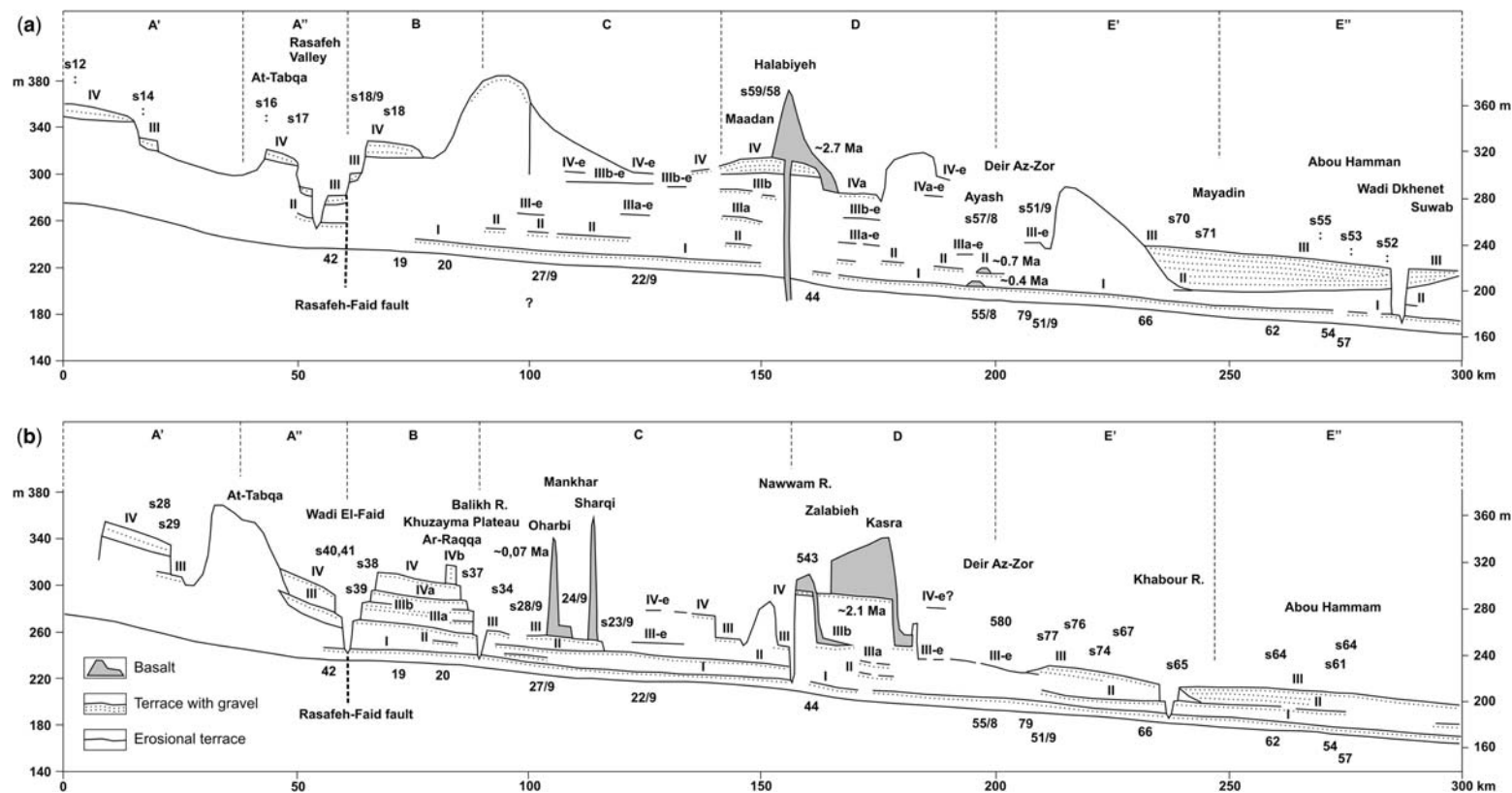
Fig. 5. Longitudinal geomorphological profiles along the southwestern (a) and the northeastern (b) sides of the Euphrates valley.
