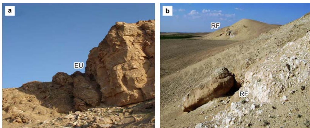
Fig. 4. Neotectonic features of the Euphrates valley: (a) the Euphrates Fault (EU) as a scarp cutting the Tortonian on the rear side of the terrace I opposite the town of Ar Raqqa (s 19/9); (b) the Rasafeh–El Faïd fault zone (RF) cutting the Tortonian on the southern side of the Euphrates valley (s 18/9). Photographs by V. G. Trifonov.
