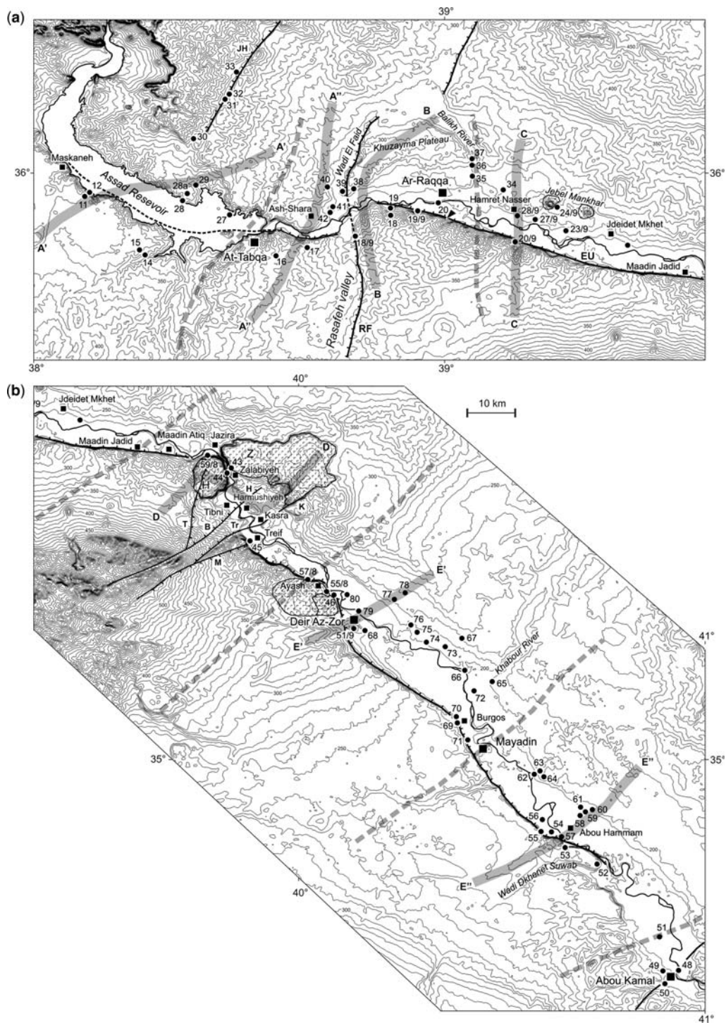
Fig. 2. The Euphrates valley between the Assad Reservoir and the town of Abou Kamal. B continues A to the SE. The map demonstrates isohypses with the 10 m interval according to the Shuttle Radar Topography Mission (SRTM) data and the location of Late Cenozoic faults, basaltic fields, sites of our observations and some trigpoints. The Euphrates
