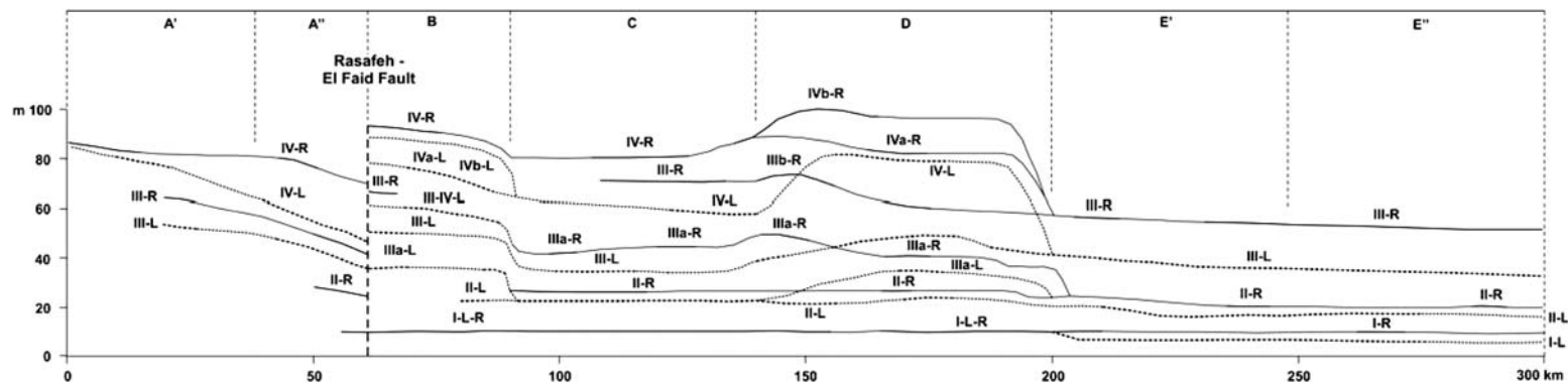
Fig. 6. Geomorphological profile along the Euphrates valley, based on combined evidence; 'r' is the right bank and 'l' is the left bank of the valley.
