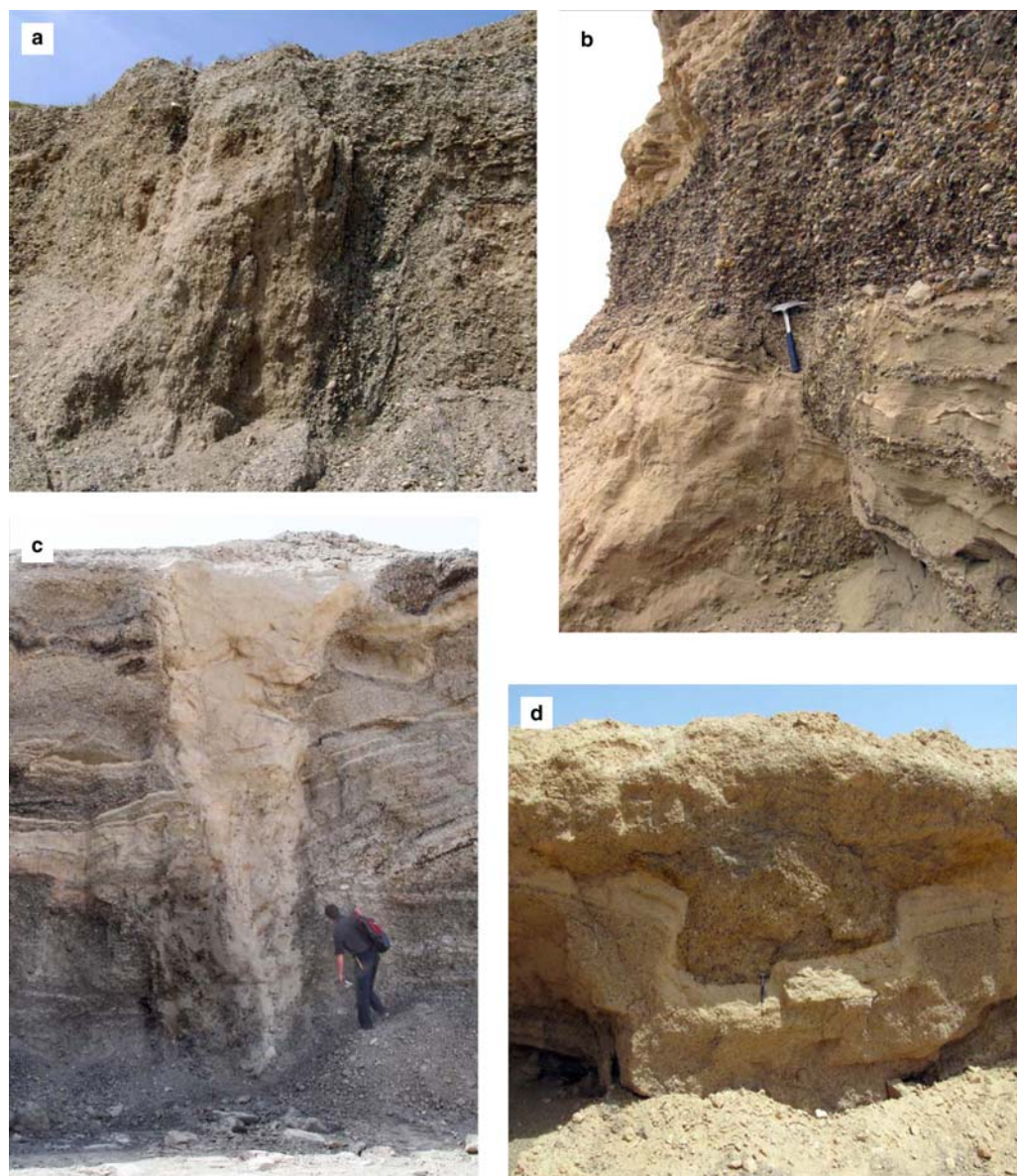
Fig. 8. Sand and gravel dykes and secondary tectonic deformation affected terrace alluvium. (a) Gravel dyke cutting terrace III b on the eastern side of the Rasafeh–El Faïd fault zone, left bank of Euphrates (s 38); (b) reverse micro-fault cutting terrace II on the northeastern pericline of the Bishri anticline, the right bank of Euphrates near the village of Treif (s 45); (c) sand dyke cutting terrace II in the eastern part of the northeastern pericline of the Bishri anticline, the right bank of Euphrates in a quarry SE of Ayash (s 55/8); and (d) small fold in terrace II on the western side of the NE-trending fault zone, right bank of Euphrates in the town of Abou Kamal (s 49). Photographs by V. G. Trifonov.
