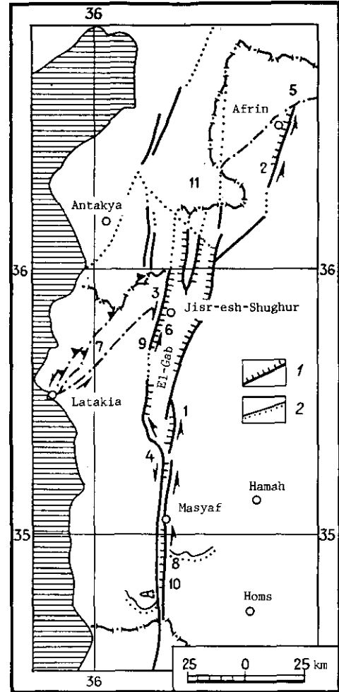
Fig. 3. Syrian segment of the Levant fault zone. 1) Faults with an upthrow component of displacement; 2) northern boundary of the field of Late Miocene plateau basalts. See Fig. 1 for other notation. Numbers on the map: 1 - ruins of Afamiya (Apamea), 2 - Dar-Taaz, 3 - Zhanudie, 4 - Jur el Ain el Kruum, 5 - Midanki, 6 - Nahr-el-Azi, 7 - Salyb-Yastin, 8 - Saraiya natural boundary, 9 - Sarmanie, 10 - Haddi, 11 - Lake Al-Umk.
