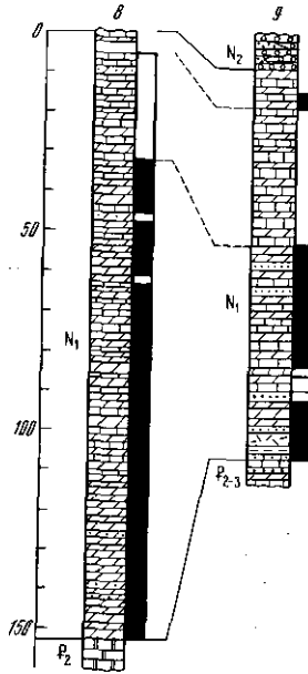
Fig. 7. Profiles of Lower Miocene deposits of the western limb of the Levant fault zone near Zhanudie (8) and the eastern limb near Midanki (9). See Fig. 5 for notation.
